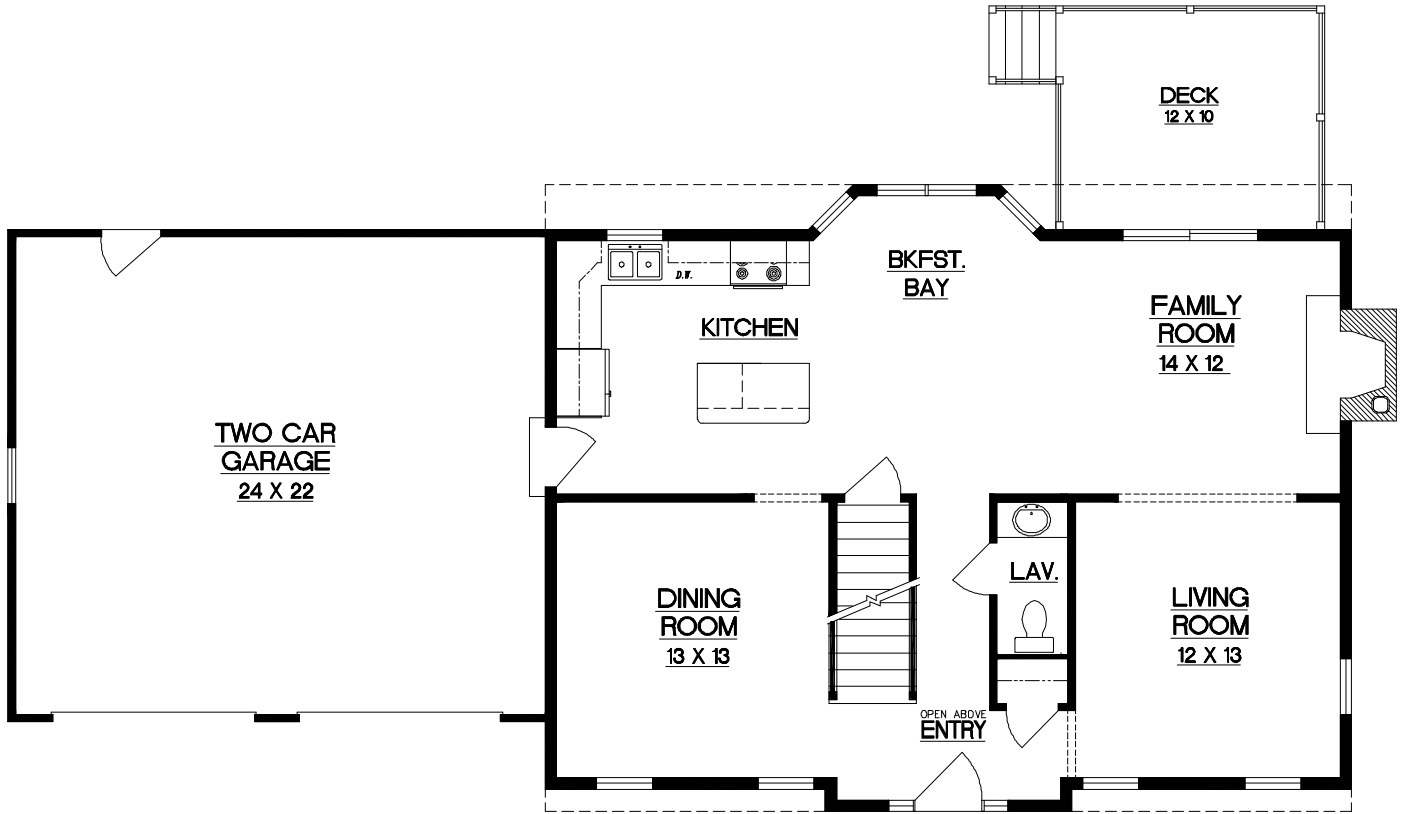
First Floor
